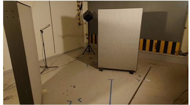
Figure 2: Two Lintex Unit 1800x1200 mm textile/textile, measured for sound absorption.
